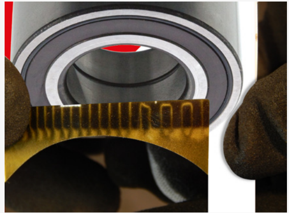
Example of a faulty reluctor using a magnetic test card
